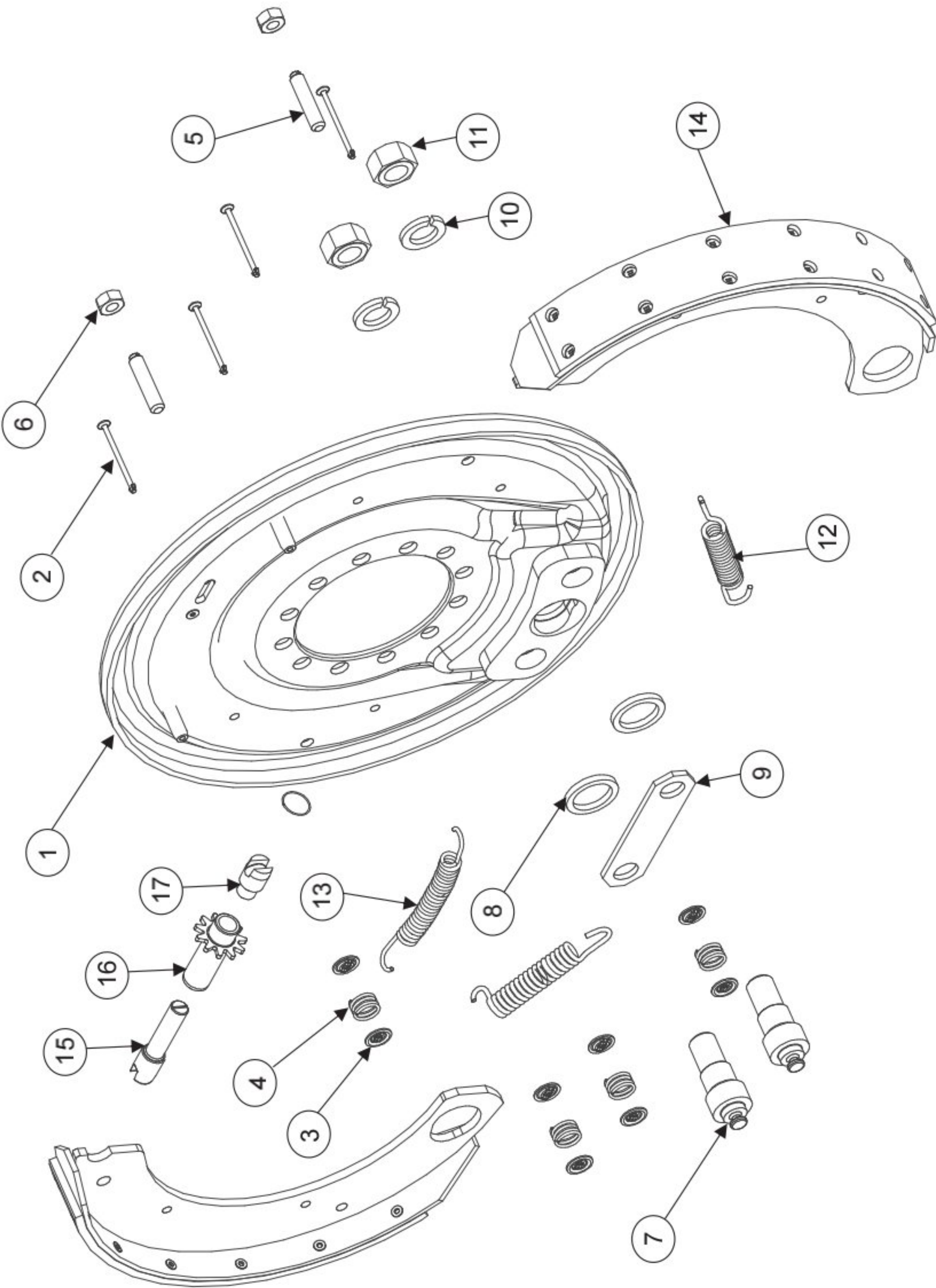
TAFE - Drum Brake Assembly - DAFC (14" x 2")
